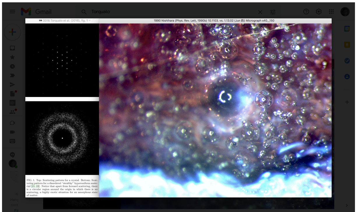
Figure 5: The scattering from a hyperuniform amorphous material shows no scattering in small angles apart from the forward peak ( https://cutt.ly/ZWyLgjk ). This is very untypical in amorphous matter and might reflect the diffraction pattern of dark photons at the magnetic body of the system.
