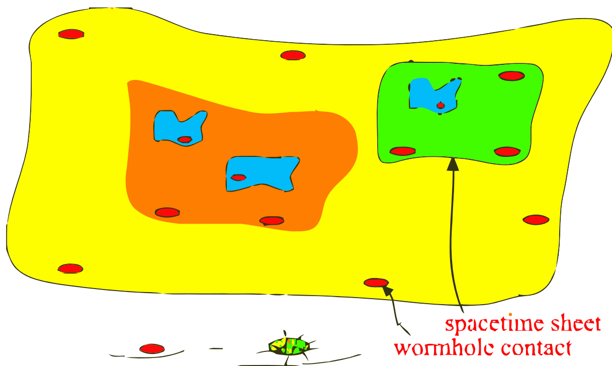
Figure 1: Many-sheeted space-time.
