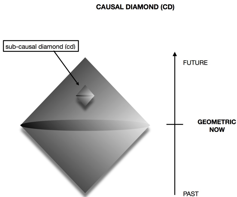
Figure 2: Causal diamond
