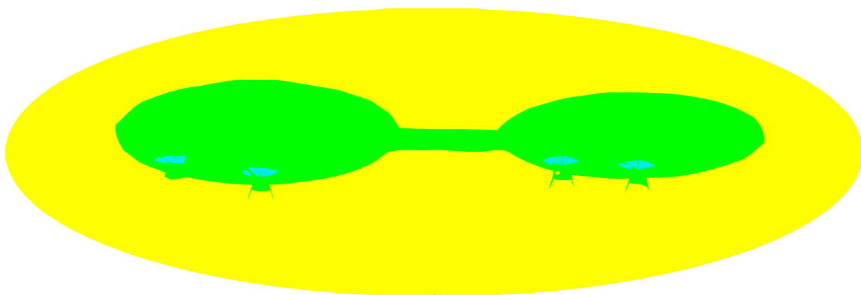
Figure 3: Wormhole contacts.
