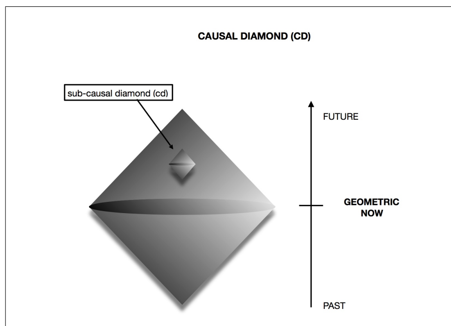
Figure 1: Causal diamond.
